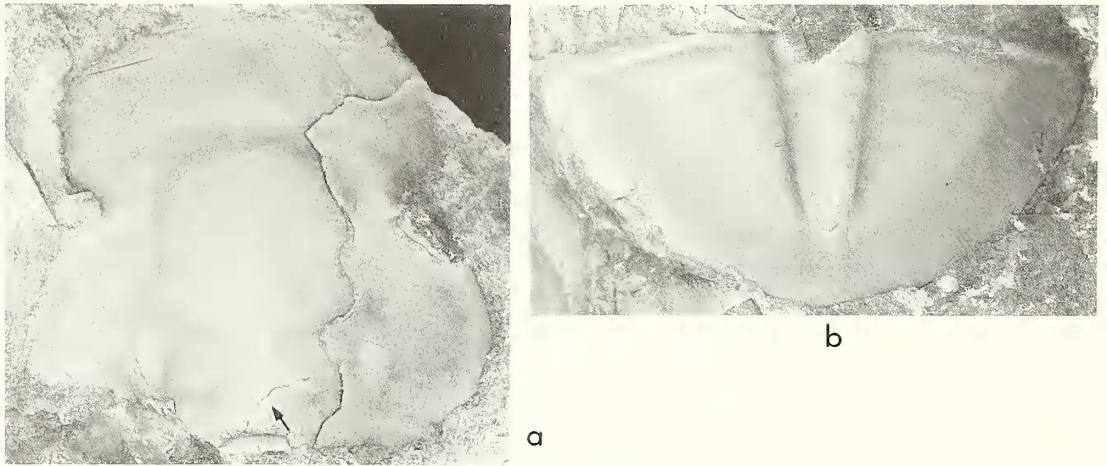
TEXT-FIG. 21. Anomocarioides limbatus (Angelin) (Middle Cambrian, Andrarum Limestone, Scania, Sweden). a , BM 1668, internal mould of cranidium showing bacculae and median glabellar tubercle (arrowed); note that, in relation to occipital furrows, this could be interpreted as pre-occipital (cf. Asaphacea), \times 4 . b , BMNH It20683, pygidium, \times 3 .
